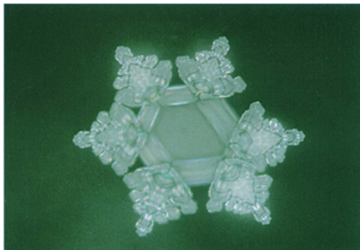
Spring water from Chuzenji Lake
