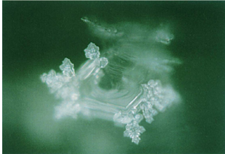
Spring water from Chuzenji Lake, treated with chlorine
