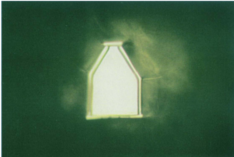
Water from a washbasin at the East entrance of the Heitate Shrine in Kumamoto prefecture
