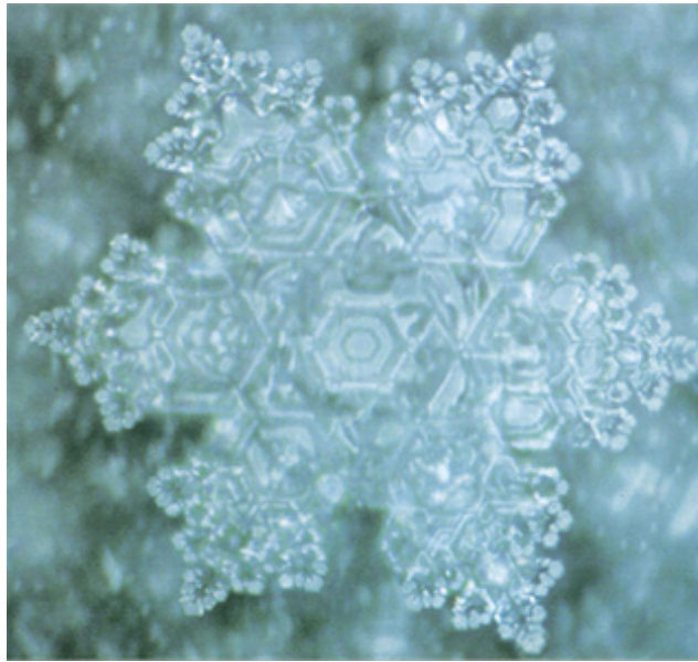
Spring water from Saijo, Hiroshima
