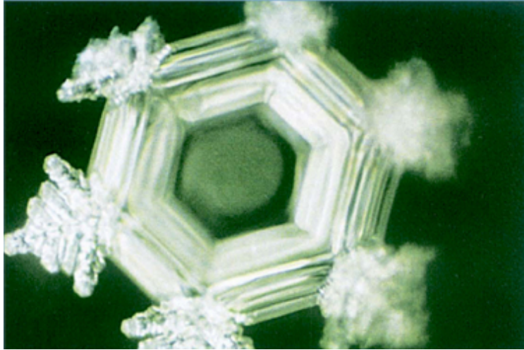
New Zealand groundwater
