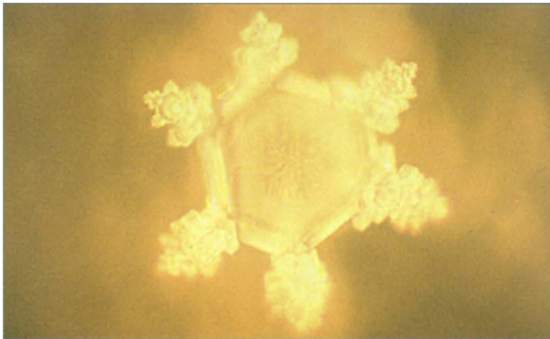
Ground water right before and after an earthquake in Shimane Prefecture, and later in the same place
